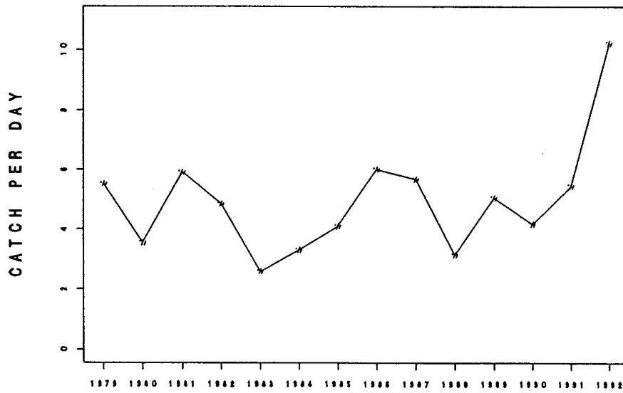
Figure 10. Yellowfin catch per day fished in the western/Japanese area
