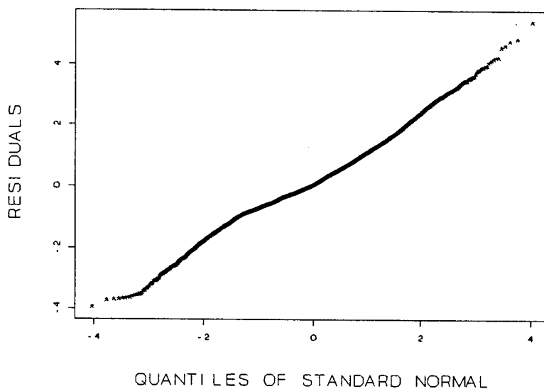
Figure 8. Residuals for the western/Japanese model versus quantiles of standard normal
