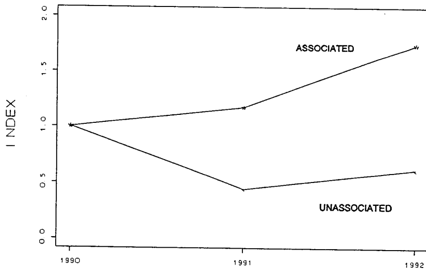
Figure 12. Indices of abundance for the eastern/American area
