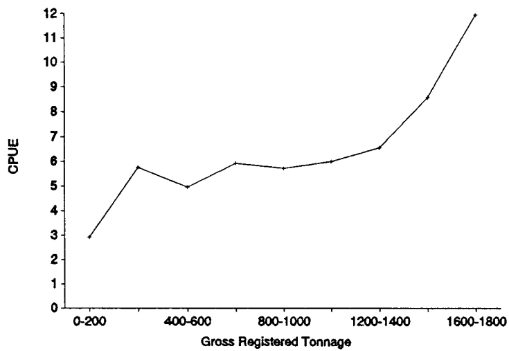
Figure 6. Yellowfin catch rate (mt per day) versus gross registered tonnage for Japanese and American purse seiners
