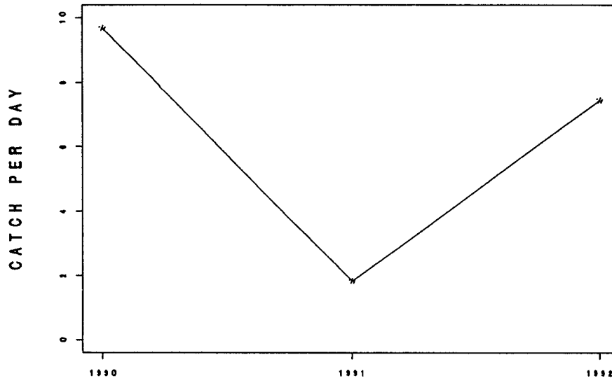
Figure 13. Yellowfin catch (mt) per day fished in the eastern/American area
