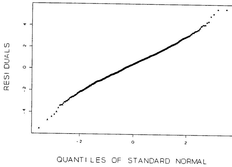
Figure 11. Residuals for the eastern/American model versus quantiles of standard normal
