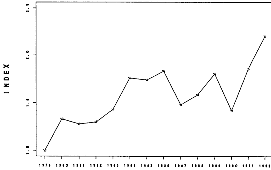
Figure 9. Indices of abundance for the western/Japanese area
