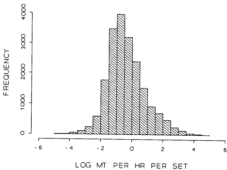
Figure 3. Frequency of transformed yellowfin catch rates
