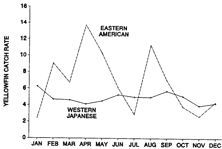
Figure 4. Yellowfin catch rate (mt per day) by month for the western/Japanese and eastern/American areas
