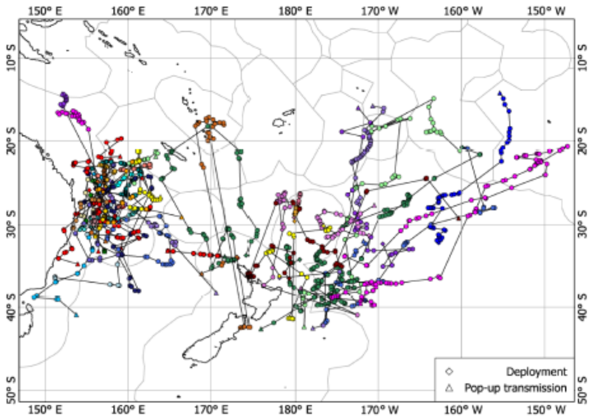
Figure 1: Position estimates of swordfish from pop-up satellite archival tags at liberty > 30 days in the south Pacific Ocean between 2006 and 2010 (reproduced from Evans et al. (2012)).
