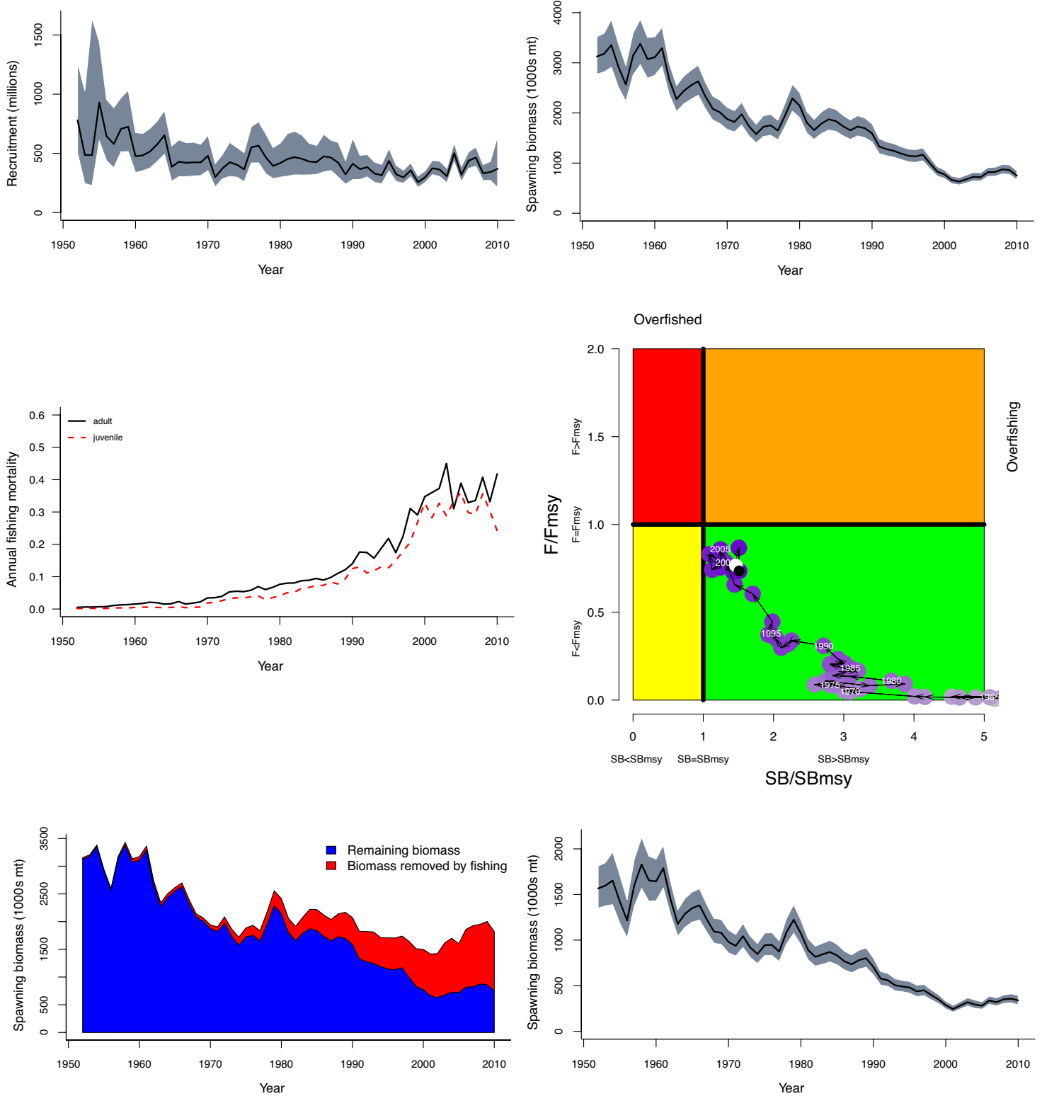
Figure 9: Estimated recruitment (top left), spawning biomass (top right), fishing mortality (middle left), stock status (middle right), estimated spawning biomass with [blue] and without [red] fishing (bottom left), and spawning biomass for the western equatorial region (bottom right) from the 2011 yellowfin tuna stock assessment.
